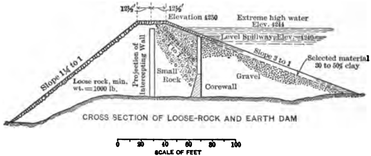
FIG. 211.—Rock-Fill Dam, Snake River, Minidoka Project, Idaho.
